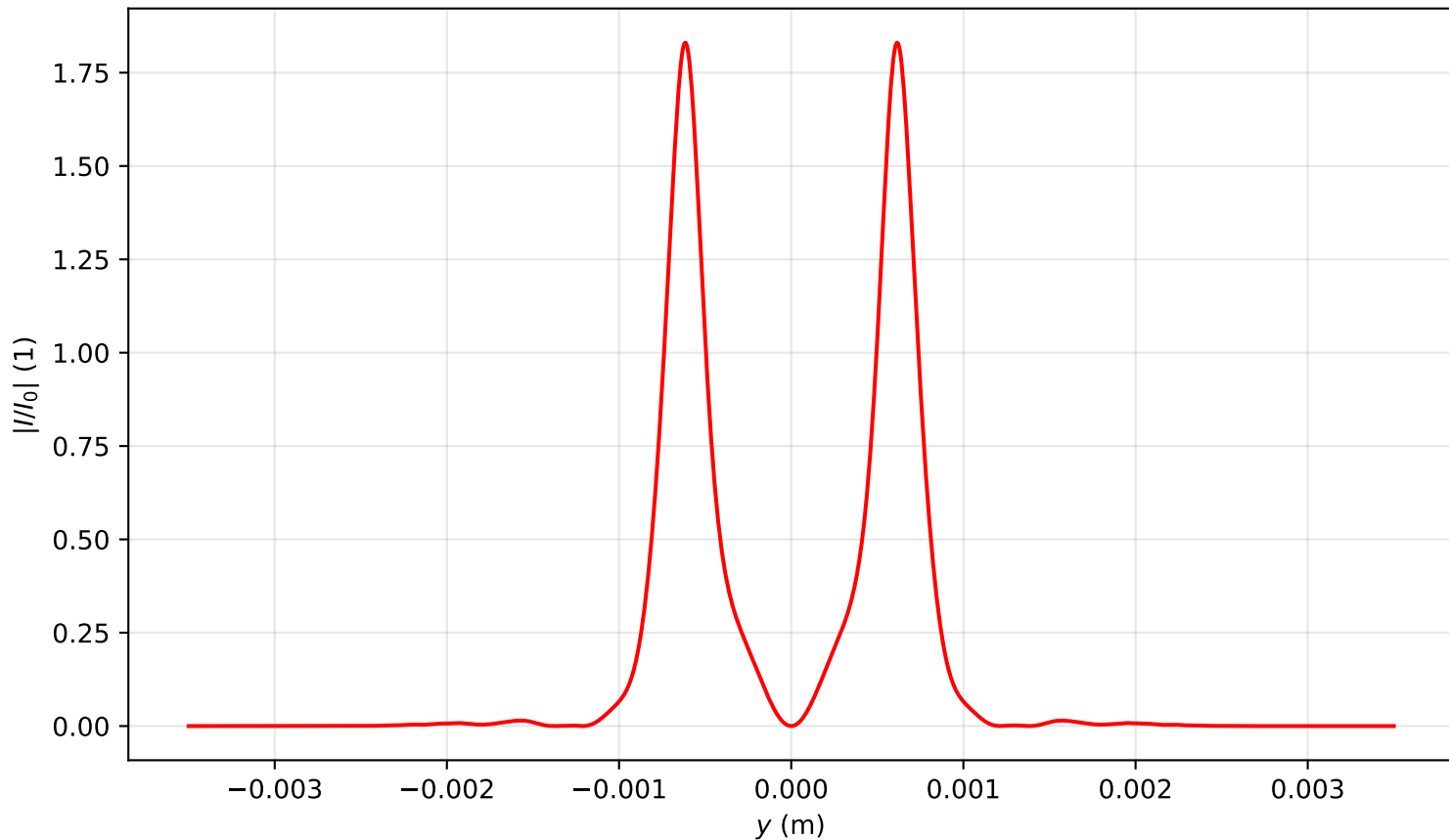
Intensity profile I(x=0, y, z=1.353)/I_0 , P_{in}=11.0P_{cr} , artificial time
