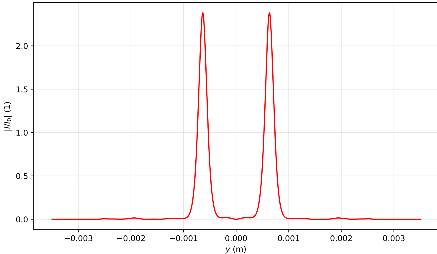
Intensity profile I(x=0, y, z=1.592)/I_0 , P_{in}=11.0P_{cr} , artificial time
