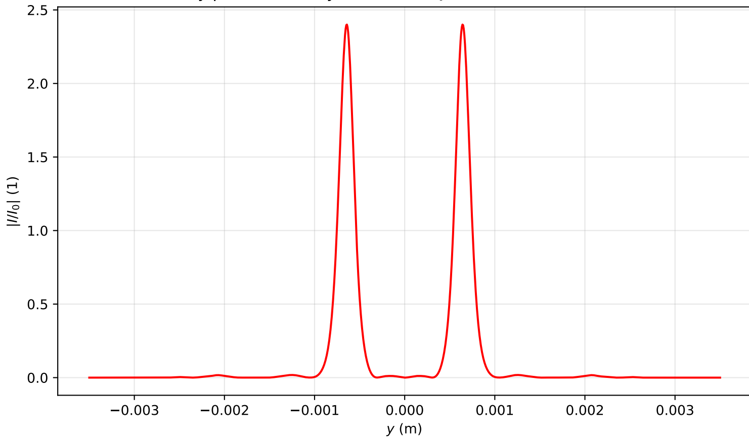
Intensity profile I(x=0, y, z=1.672)/I_0 , P_{in}=11.0P_{cr} , artificial time
