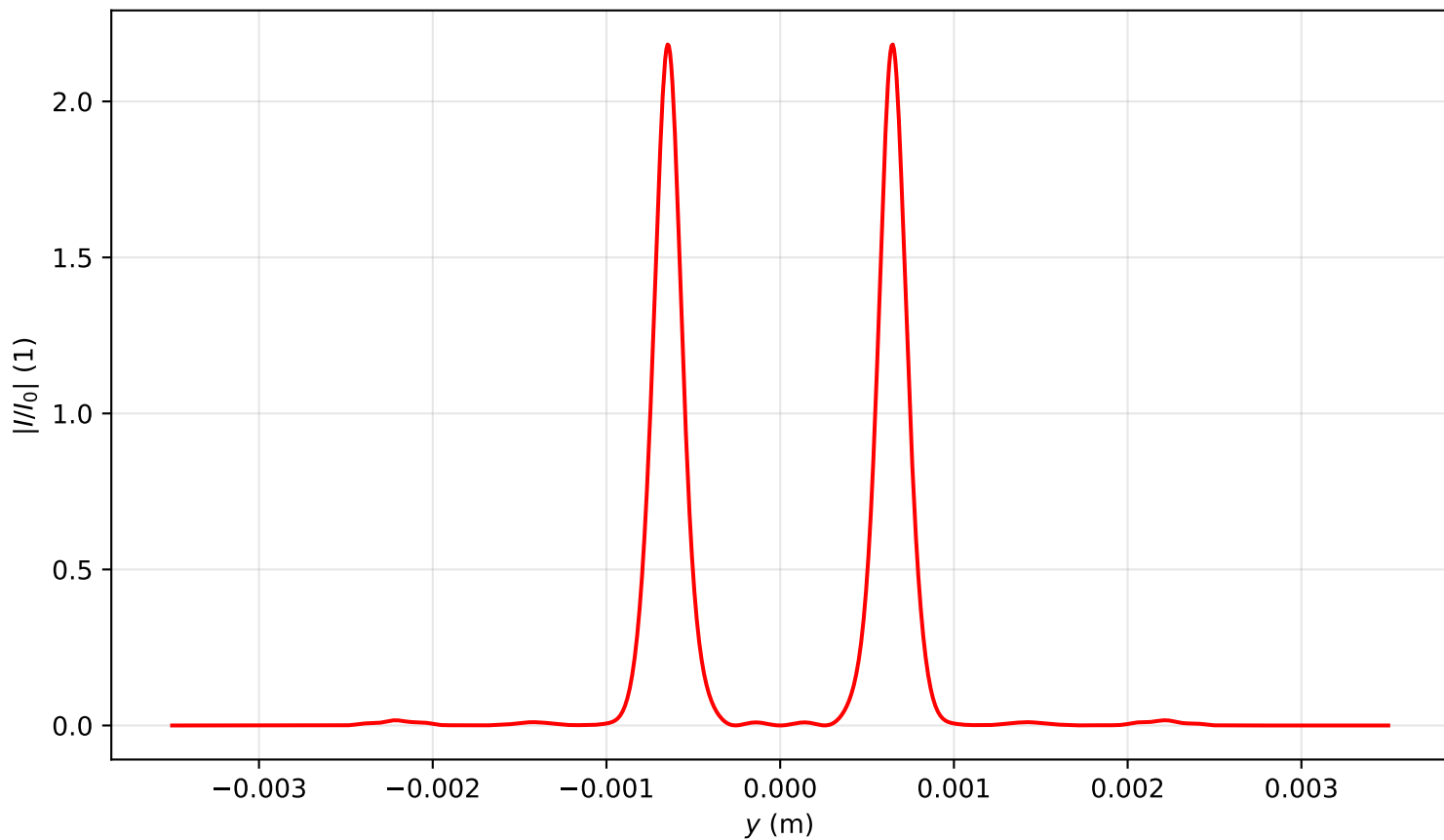
Intensity profile I(x=0, y, z=1.751)/I_0 , P_{in}=11.0P_{cr} , artificial time
