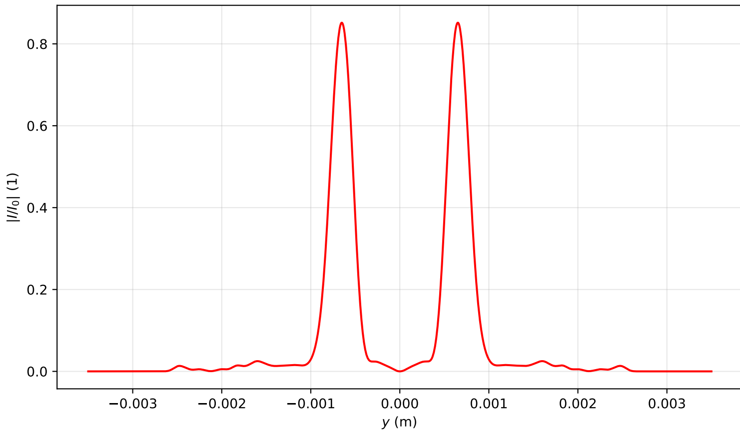
Intensity profile I(x=0, y, z=1.990)/I_0 , P_{in}=11.0P_{cr} , artificial time
