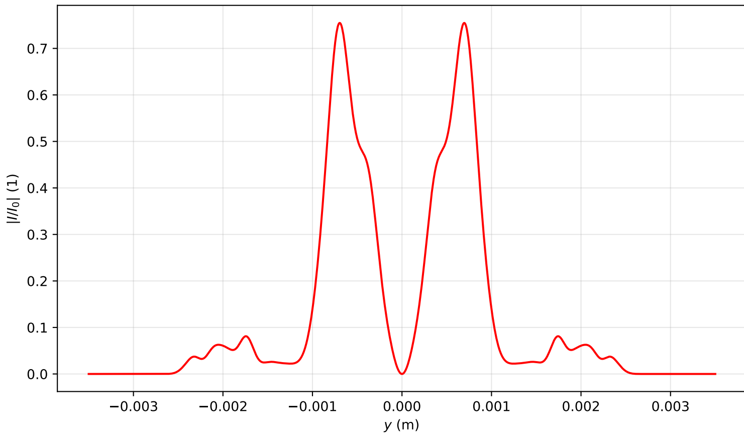
Intensity profile I(x=0, y, z=2.468)/I_0 , P_{in}=11.0P_{cr} , artificial time
