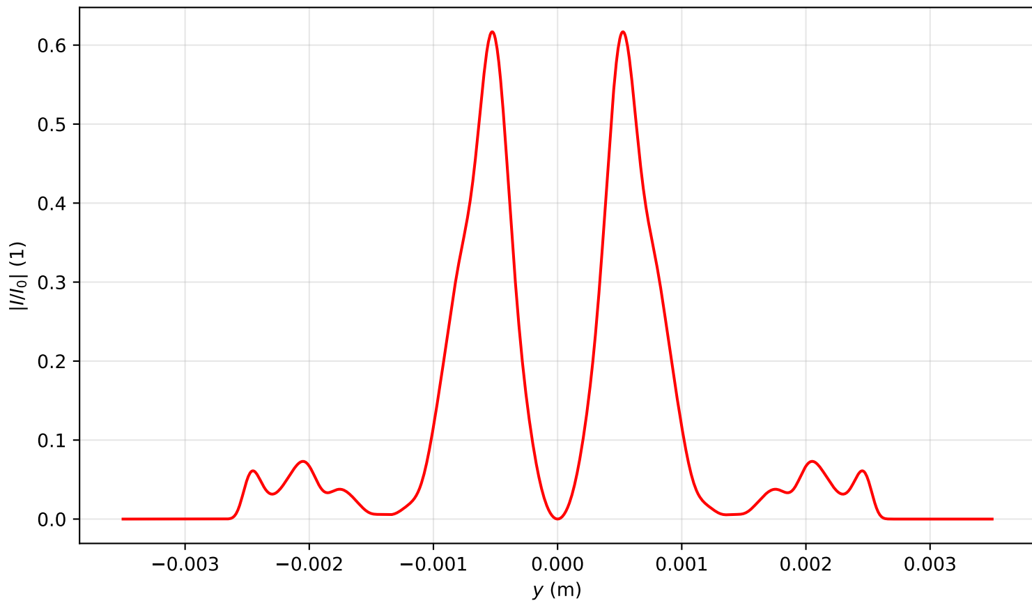
Intensity profile I(x=0, y, z=2.627)/I_0 , P_{in}=11.0P_{cr} , artificial time
