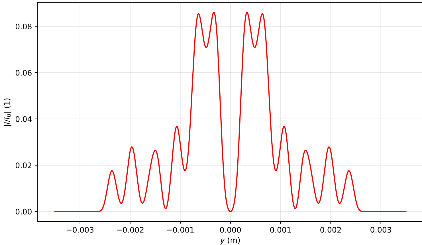
Intensity profile I(x=0, y, z=3.742)/I_0 , P_{in}=11.0P_{cr} , artificial time
