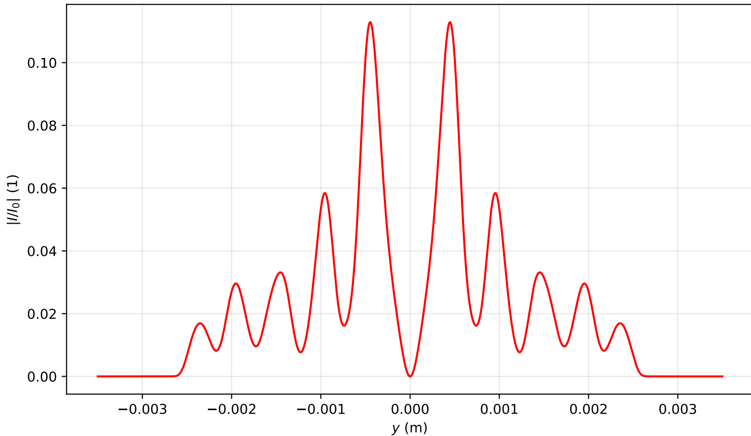
Intensity profile I(x=0, y, z=3.901)/I_0 , P_{in}=11.0P_{cr} , artificial time
