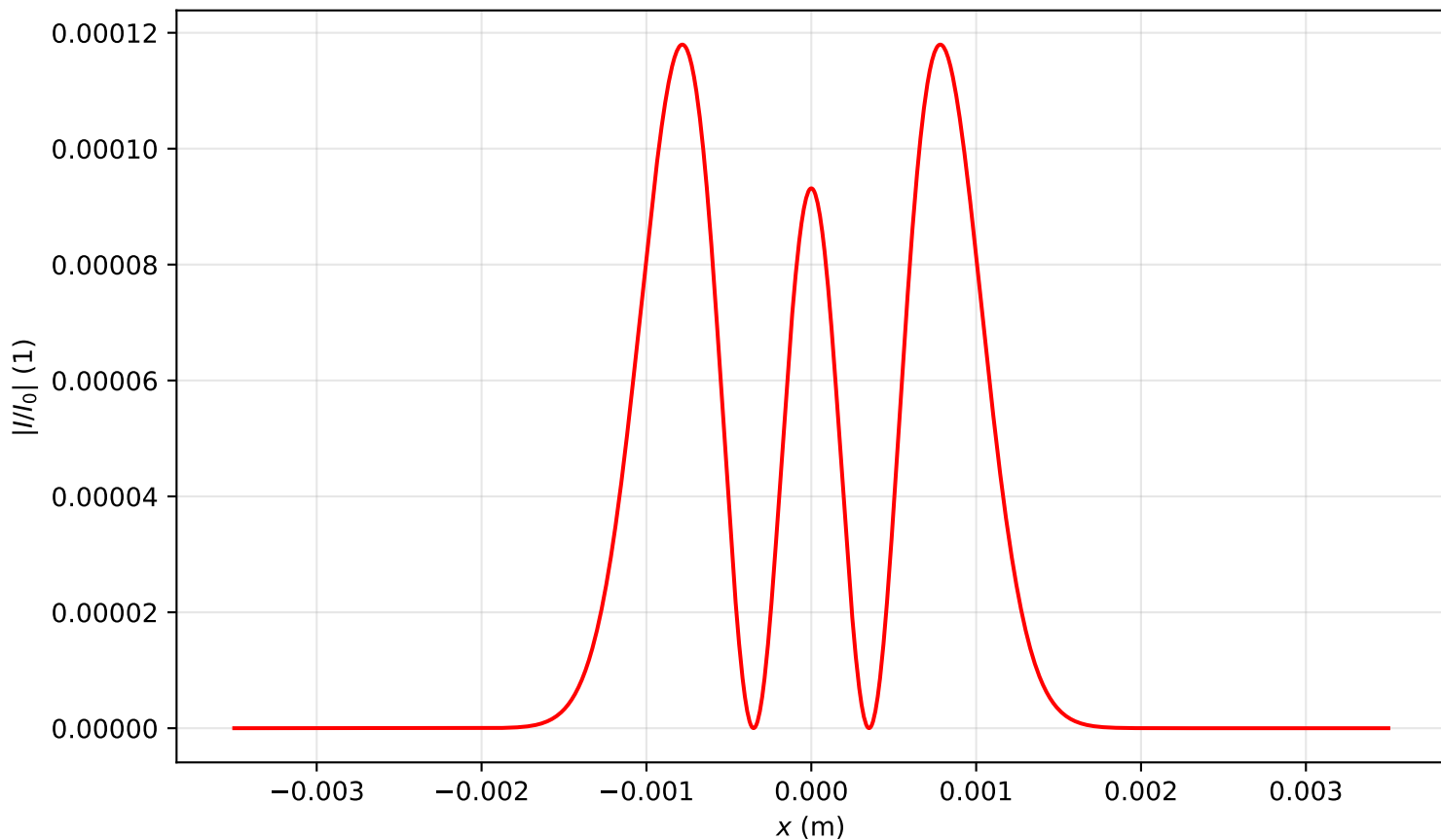
Intensity profile I(x, y = 0, z = 0.080)/I_0 , P_{in}=12.0P_{cr} , artificial time
