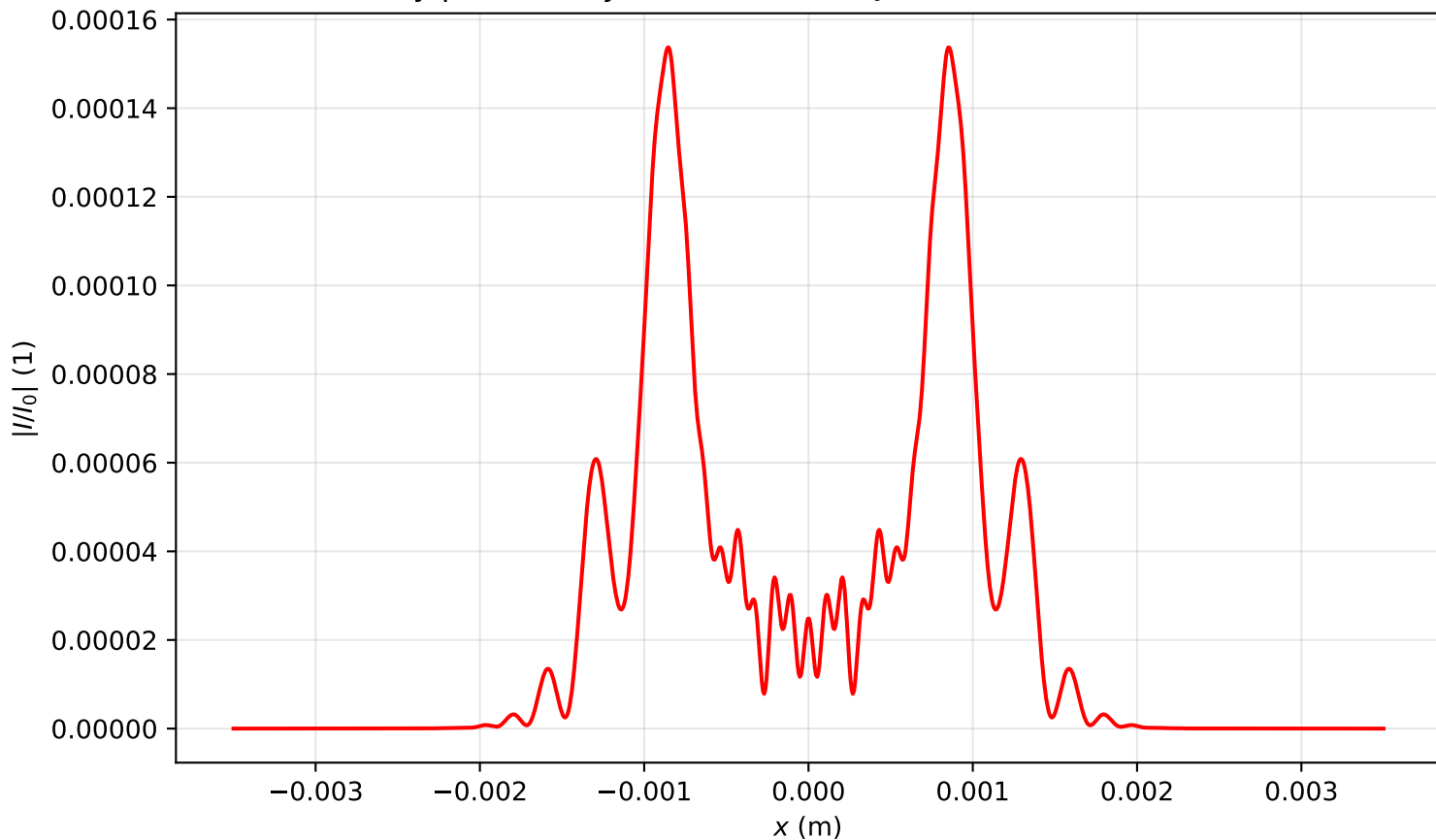
Intensity profile I(x, y = 0, z = 0.557)/I_0 , P_{in}=12.0P_{cr} , artificial time
