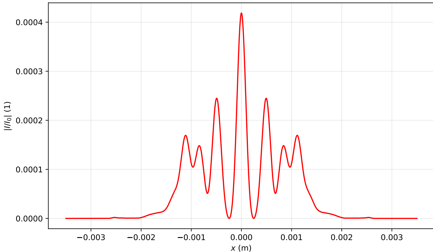
Intensity profile I(x, y = 0, z = 1.035)/I_0 , P_{in}=12.0P_{cr} , artificial time
