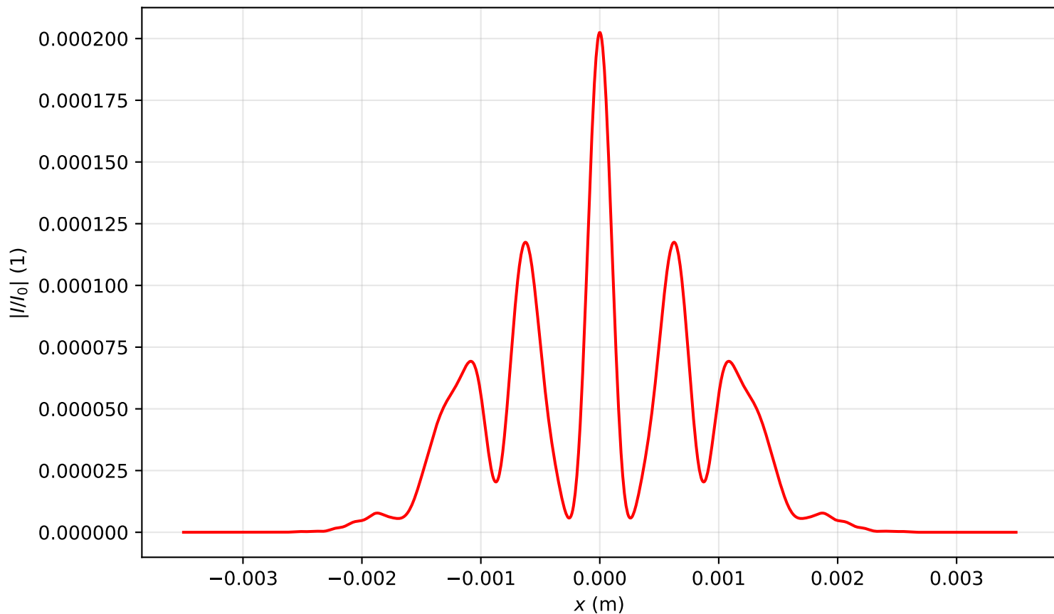
Intensity profile I(x, y = 0, z = 1.194)/I_0 , P_{in}=12.0\text{Pcr} , artificial time
