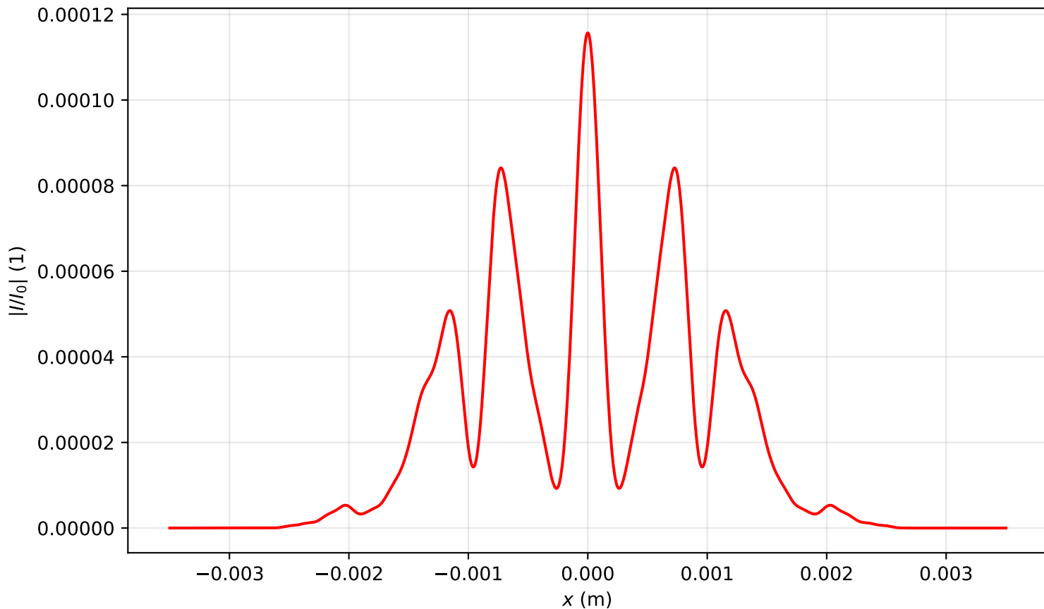
Intensity profile I(x, y = 0, z = 1.274)/I_0 , P_{in}=12.0P_{cr} , artificial time
