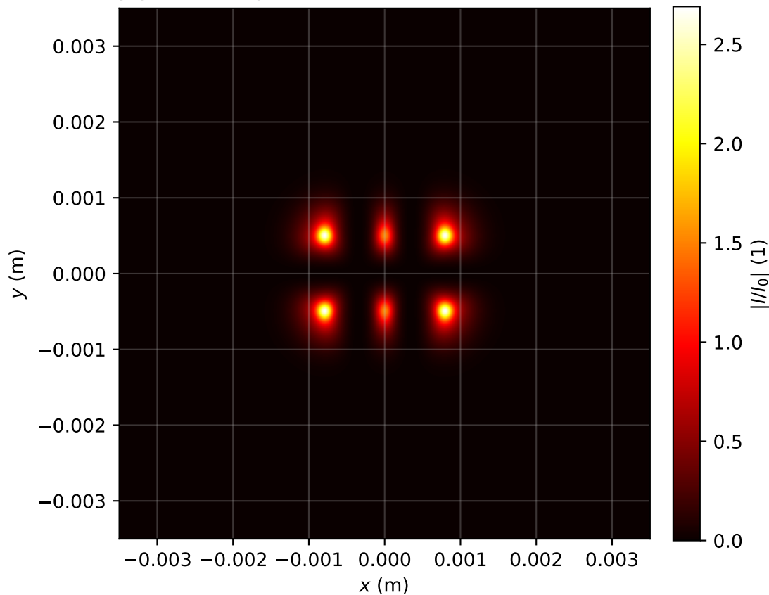
Intensity profile I(x, y, z = 0.239)/I_0 , P_{in}=12.0\text{Pcr} , artificial time
