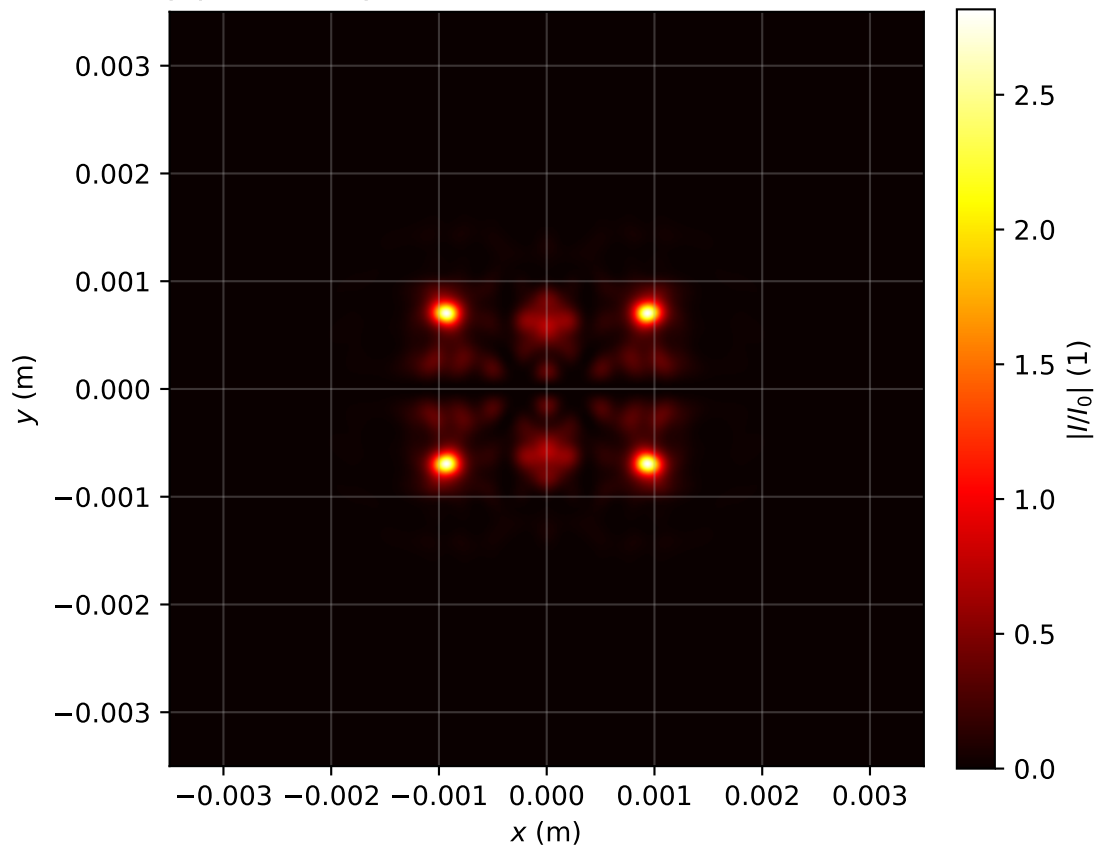
Intensity profile I(x, y, z = 1.035)/I_0 , P_{in}=12.0\text{Pcr} , artificial time
