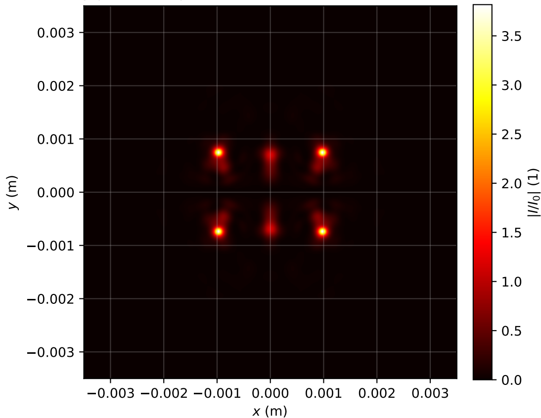
Intensity profile I(x, y, z = 1.353)/I_0 , P_{in}=12.0\text{Pcr} , artificial time
