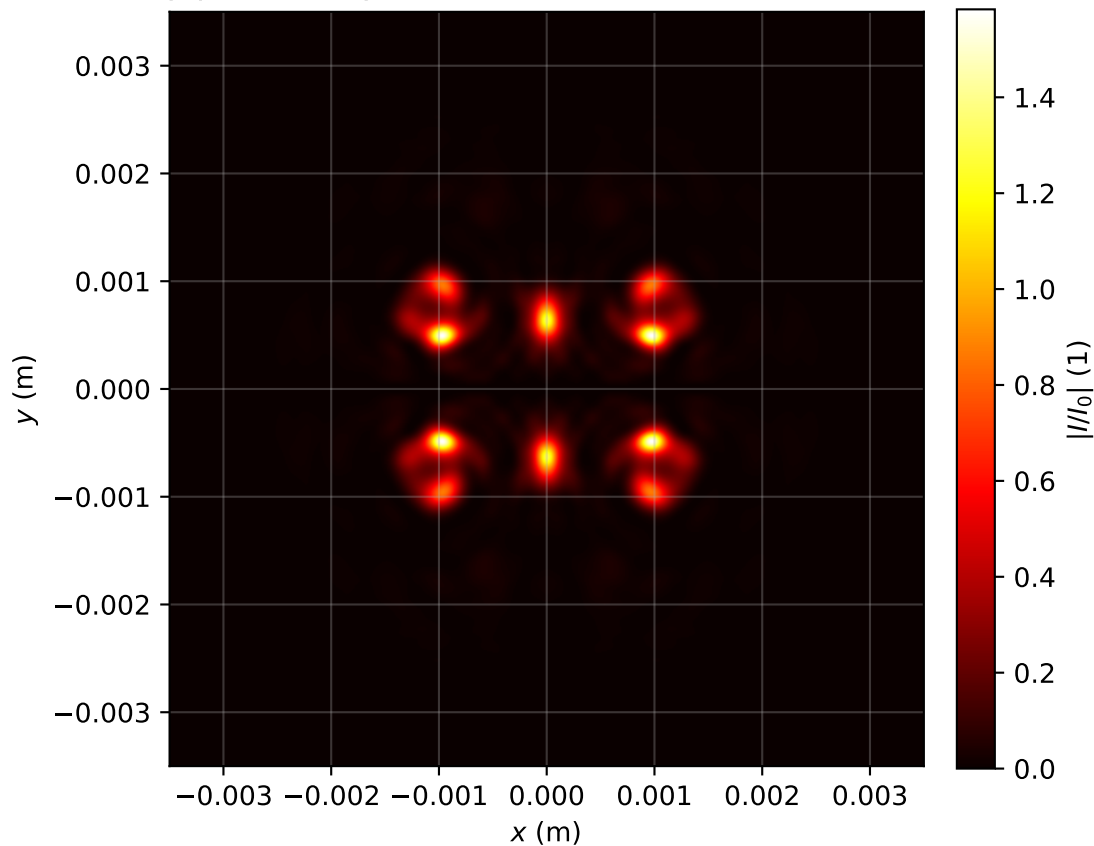
Intensity profile I(x, y, z = 1.513)/I_0 , P_{in}=12.0\text{Pcr} , artificial time
