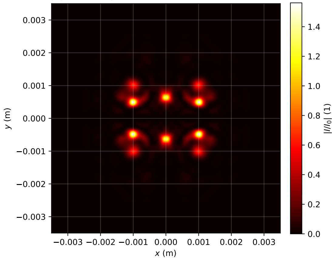
Intensity profile I(x, y, z = 1.592)/I_0 , P_{in}=12.0\text{Pcr} , artificial time
