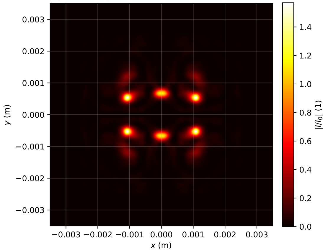
Intensity profile I(x, y, z = 1.831)/I_0 , P_{in}=12.0\text{Pcr} , artificial time
