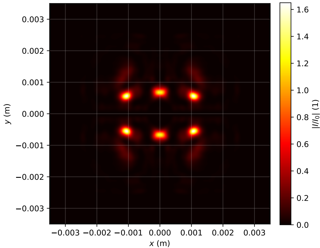
Intensity profile I(x, y, z = 1.911)/I_0 , P_{in}=12.0\text{Pcr} , artificial time
