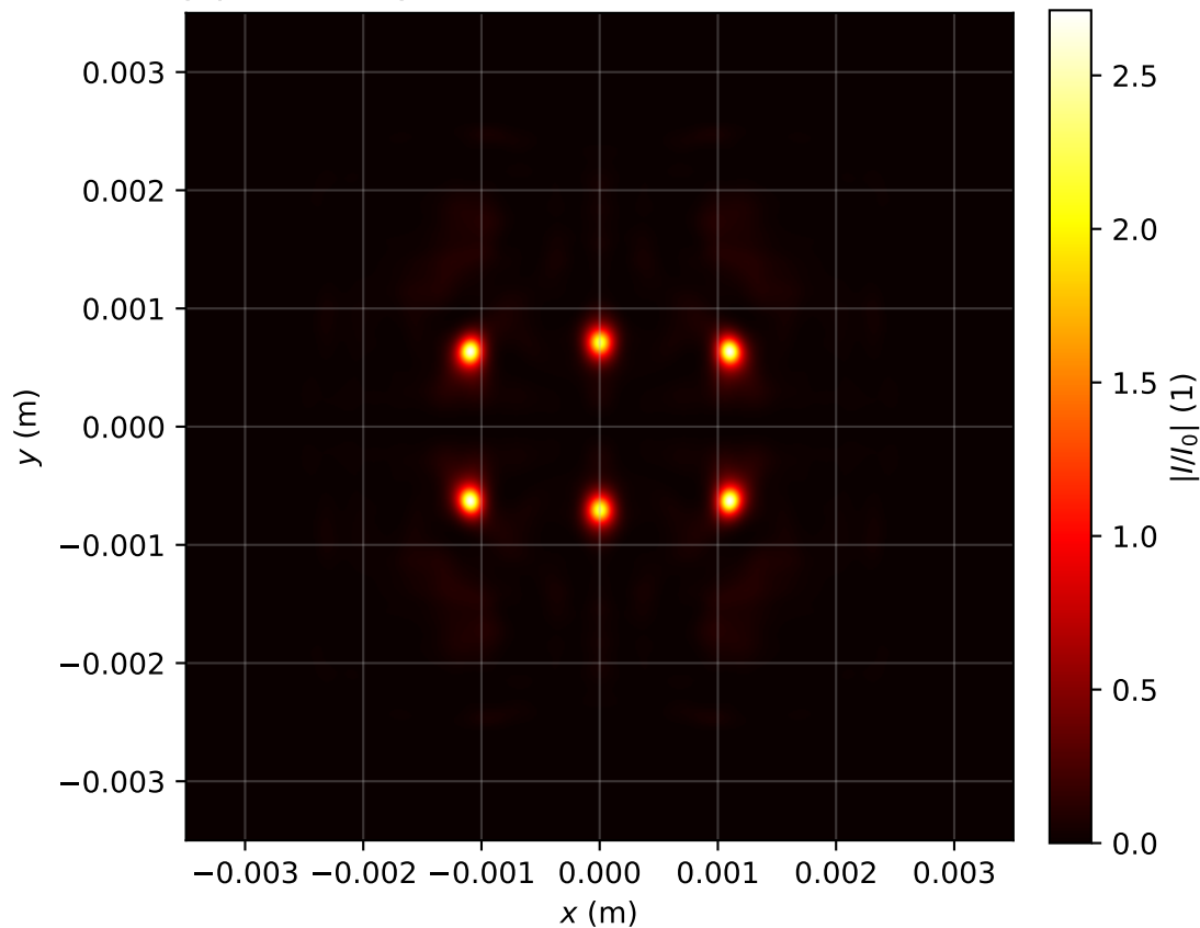
Intensity profile I(x, y, z = 2.149)/I_0 , P_{in}=12.0\text{Pcr} , artificial time
