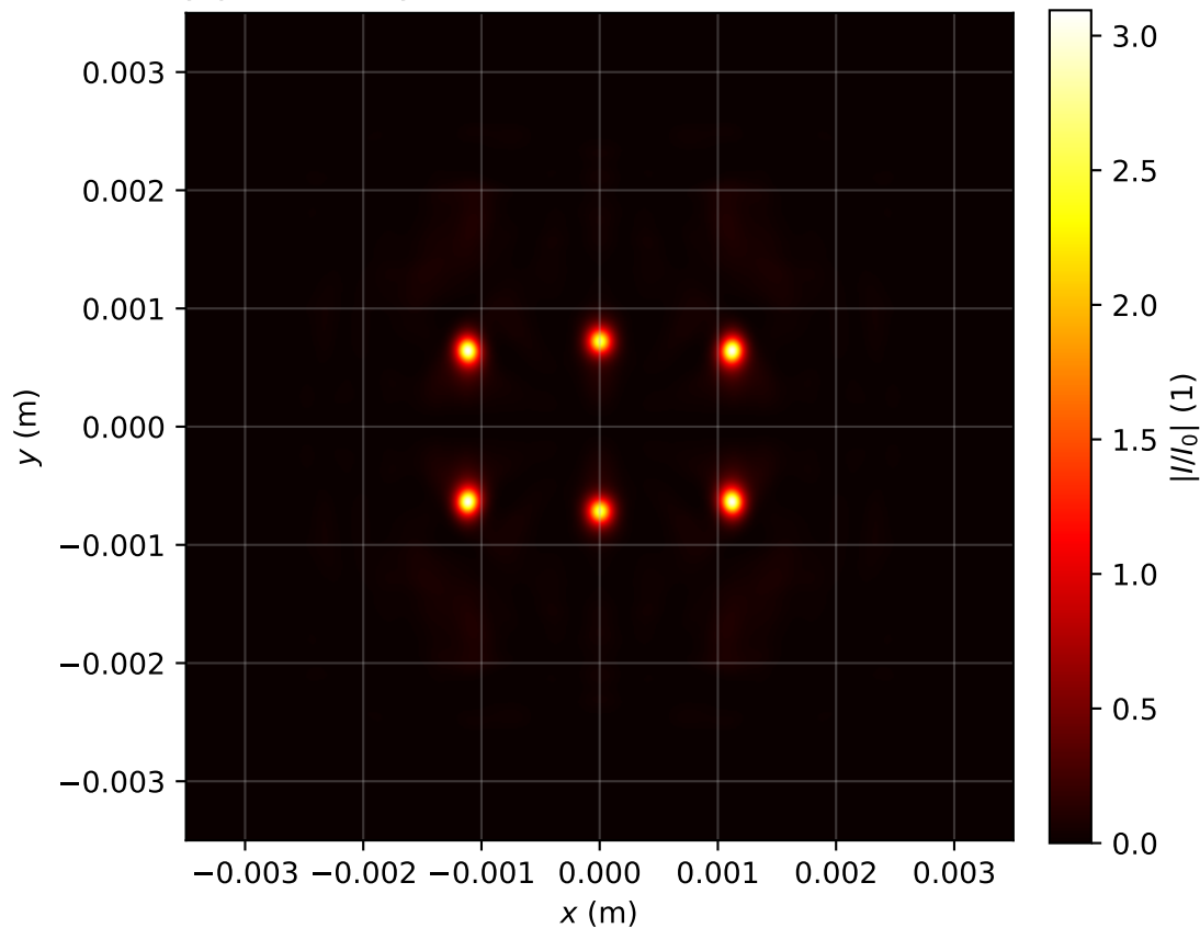
Intensity profile I(x, y, z = 2.229)/I_0 , P_{in}=12.0\text{Pcr} , artificial time
