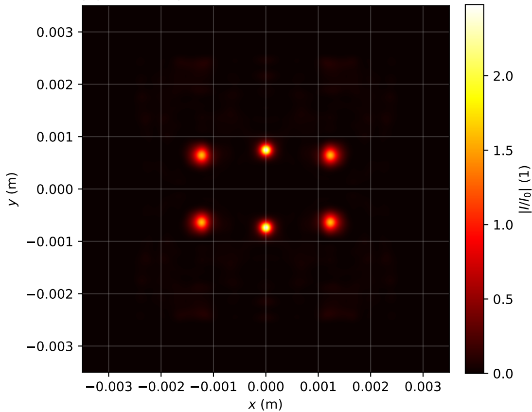
Intensity profile I(x, y, z = 2.786)/I_0 , P_{in}=12.0P_{cr} , artificial time
