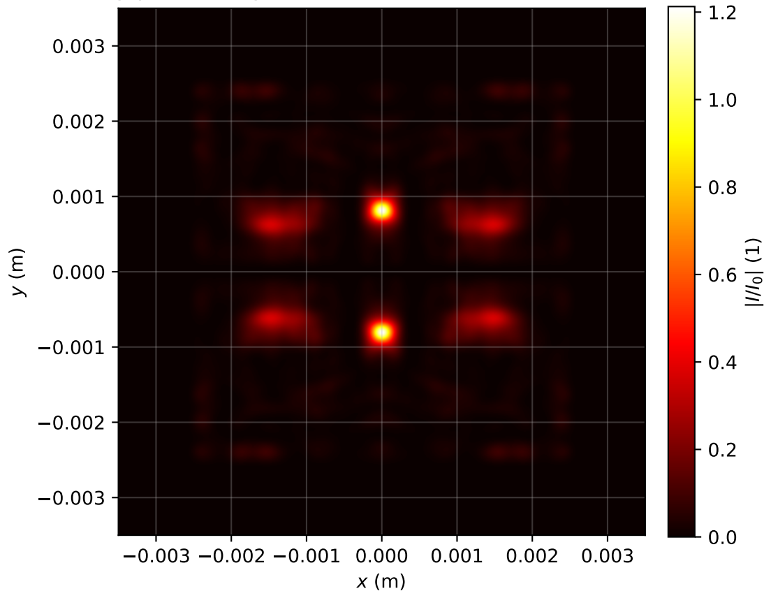
Intensity profile I(x, y, z = 3.344)/I_0 , P_{in}=12.0\text{Pcr} , artificial time
