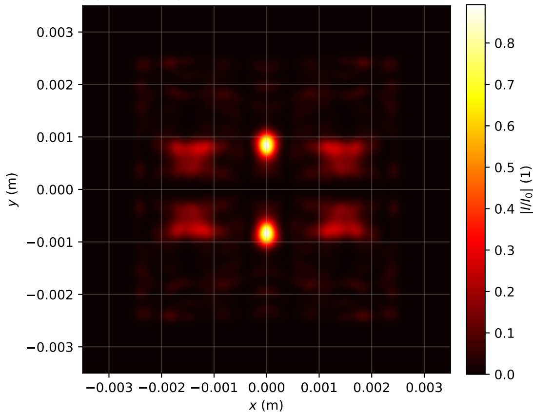
Intensity profile I(x, y, z = 3.503)/I_0 , P_{in}=12.0\text{Pcr} , artificial time
