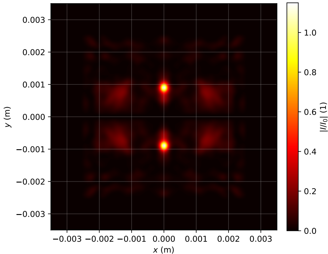
Intensity profile I(x, y, z = 3.742)/I_0 , P_{in}=12.0P_{cr} , artificial time
