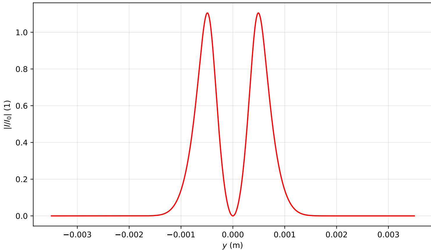
Intensity profile I(x=0, y, z=0.159)/I_0 , P_{in}=12.0P_{cr} , artificial time
