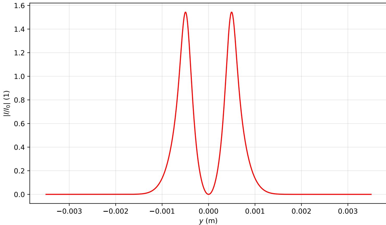
Intensity profile I(x=0, y, z=0.239)/I_0 , P_{in}=12.0P_{cr} , artificial time
