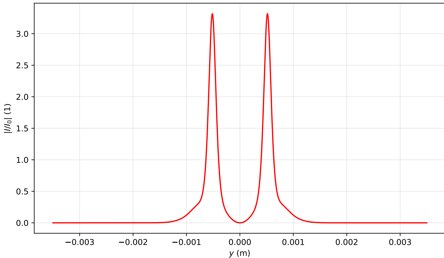
Intensity profile I(x=0, y, z=0.398)/I_0 , P_{in}=12.0P_{cr} , artificial time
