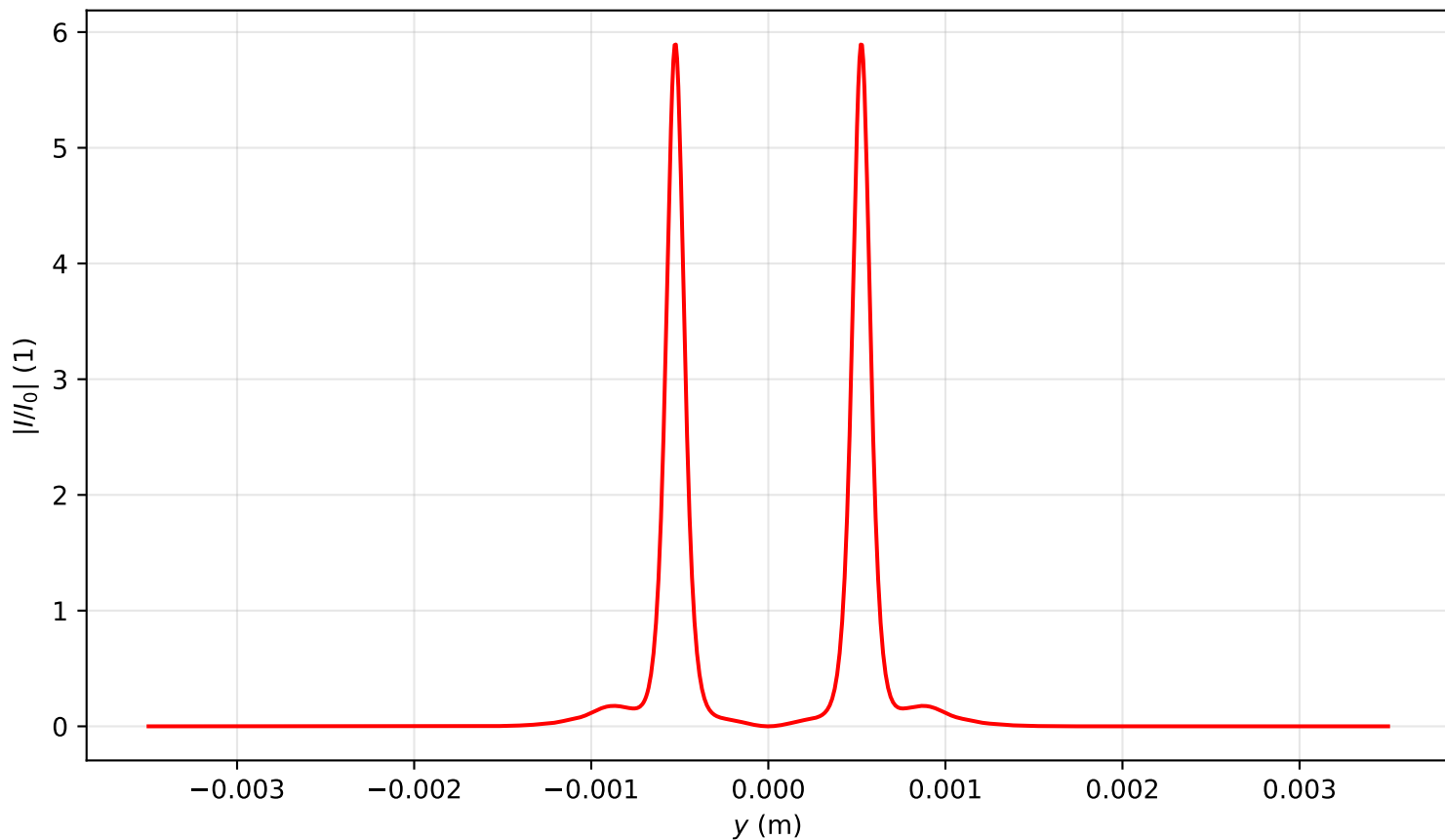
Intensity profile I(x=0, y, z=0.478)/I_0 , P_{in}=12.0\text{Pcr} , artificial time
