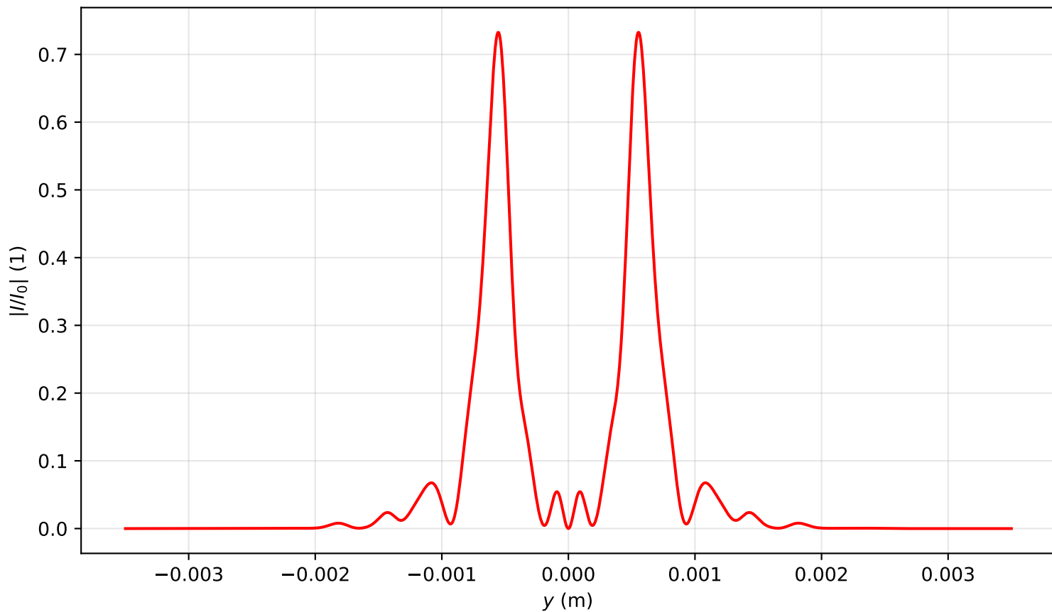
Intensity profile I(x=0, y, z=0.876)/I_0 , P_{in}=12.0P_{cr} , artificial time
