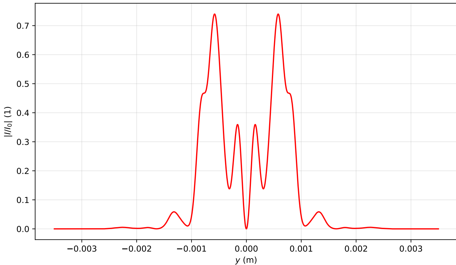
Intensity profile I(x=0, y, z=1.035)/I_0 , P_{in}=12.0P_{cr} , artificial time
