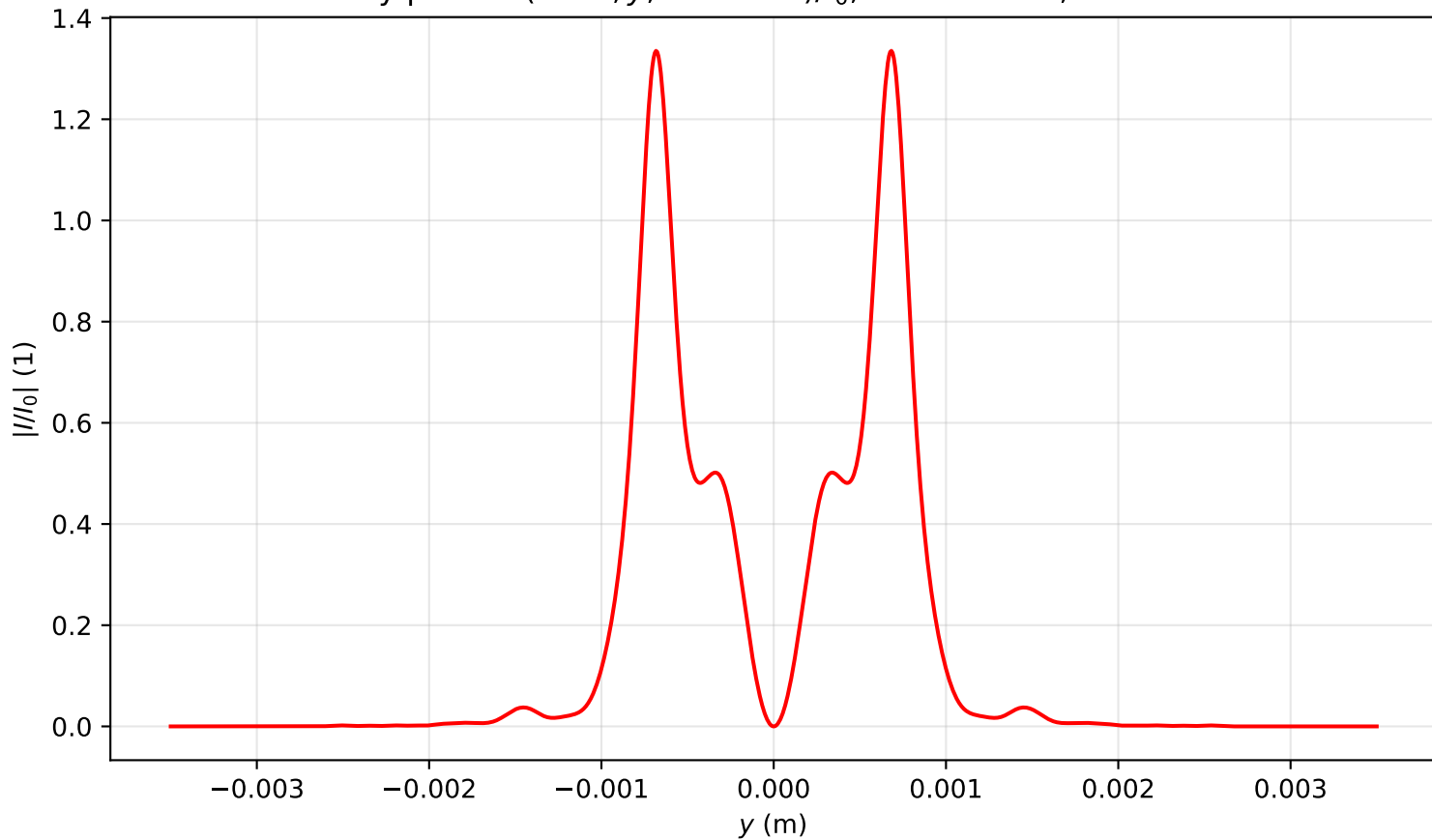
Intensity profile I(x=0, y, z=1.274)/I_0 , P_{in}=12.0P_{cr} , artificial time
