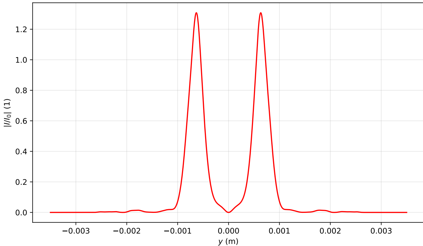
Intensity profile I(x=0, y, z=1.513)/I_0 , P_{in}=12.0P_{cr} , artificial time
