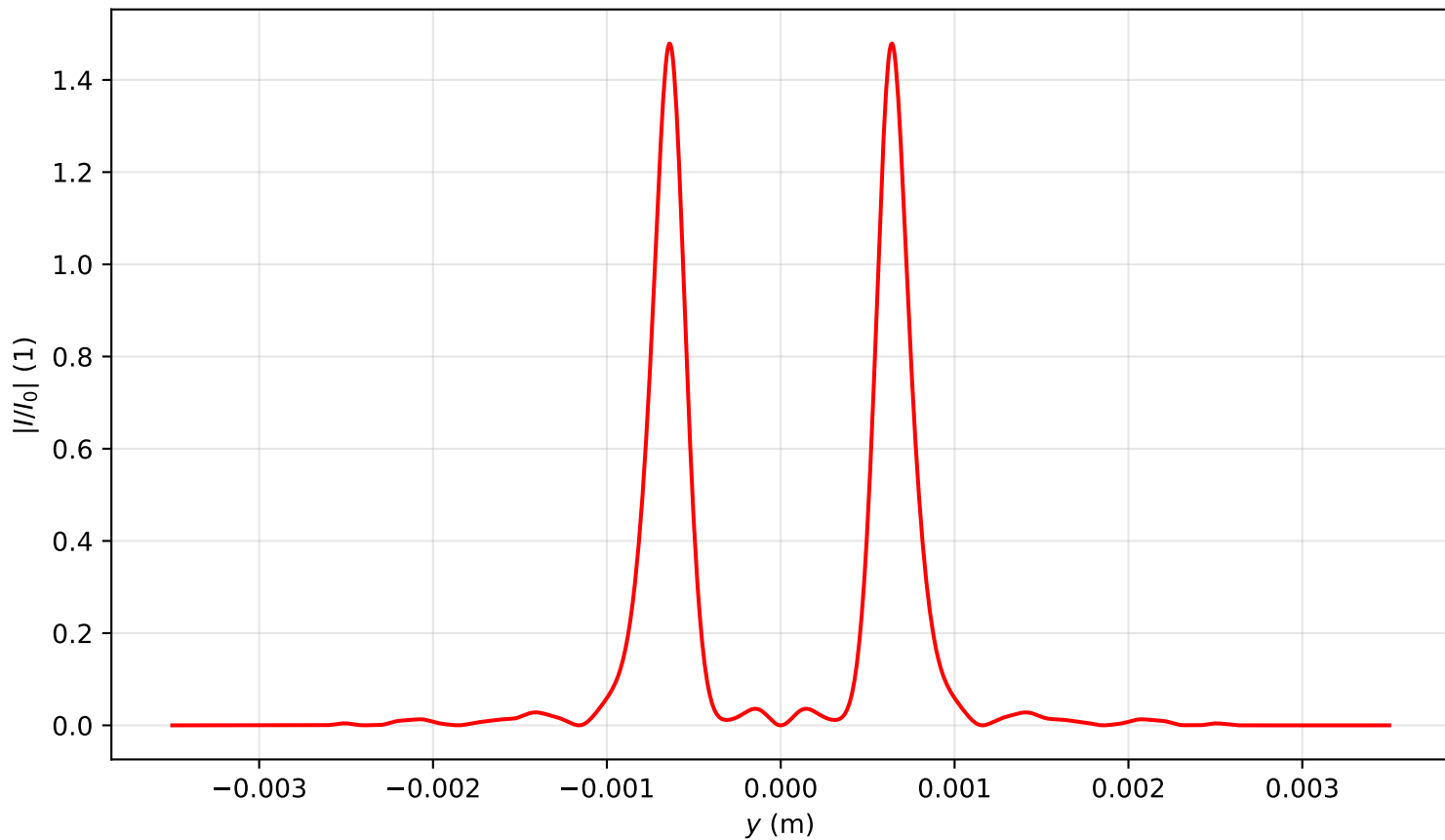
Intensity profile I(x=0, y, z=1.672)/I_0 , P_{in}=12.0P_{cr} , artificial time
