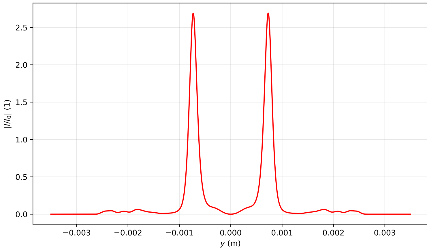
Intensity profile I(x=0, y, z=2.309)/I_0 , P_{in}=12.0P_{cr} , artificial time
