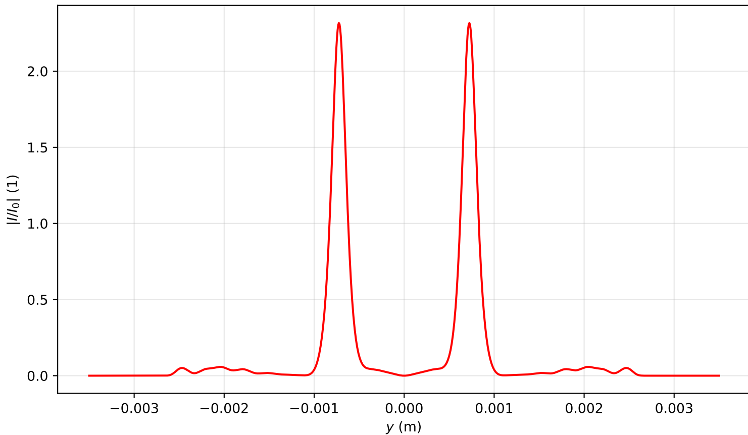
Intensity profile I(x=0, y, z=2.468)/I_0 , P_{in}=12.0P_{cr} , artificial time
