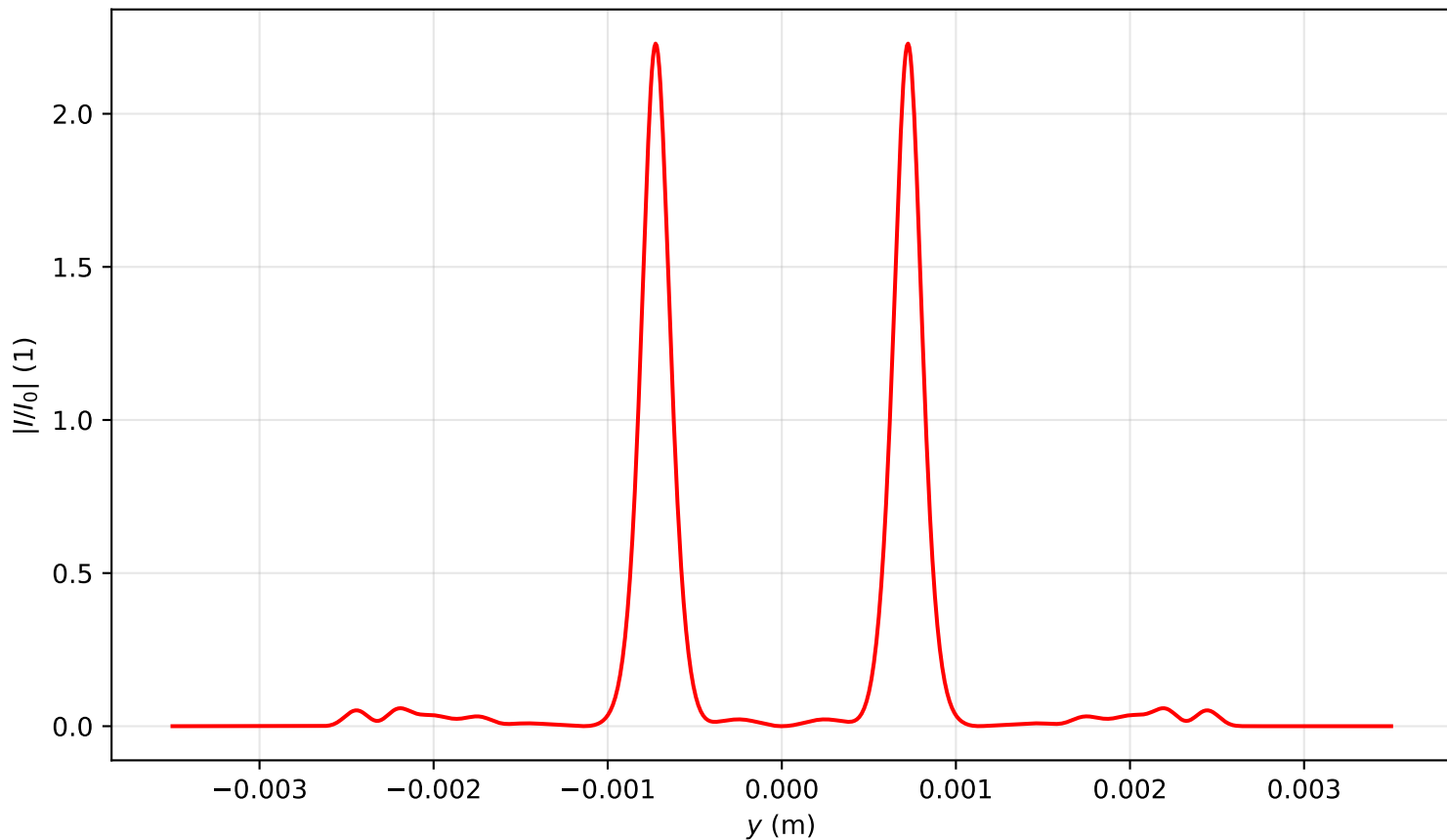
Intensity profile I(x=0, y, z=2.548)/I_0 , P_{in}=12.0P_{cr} , artificial time
