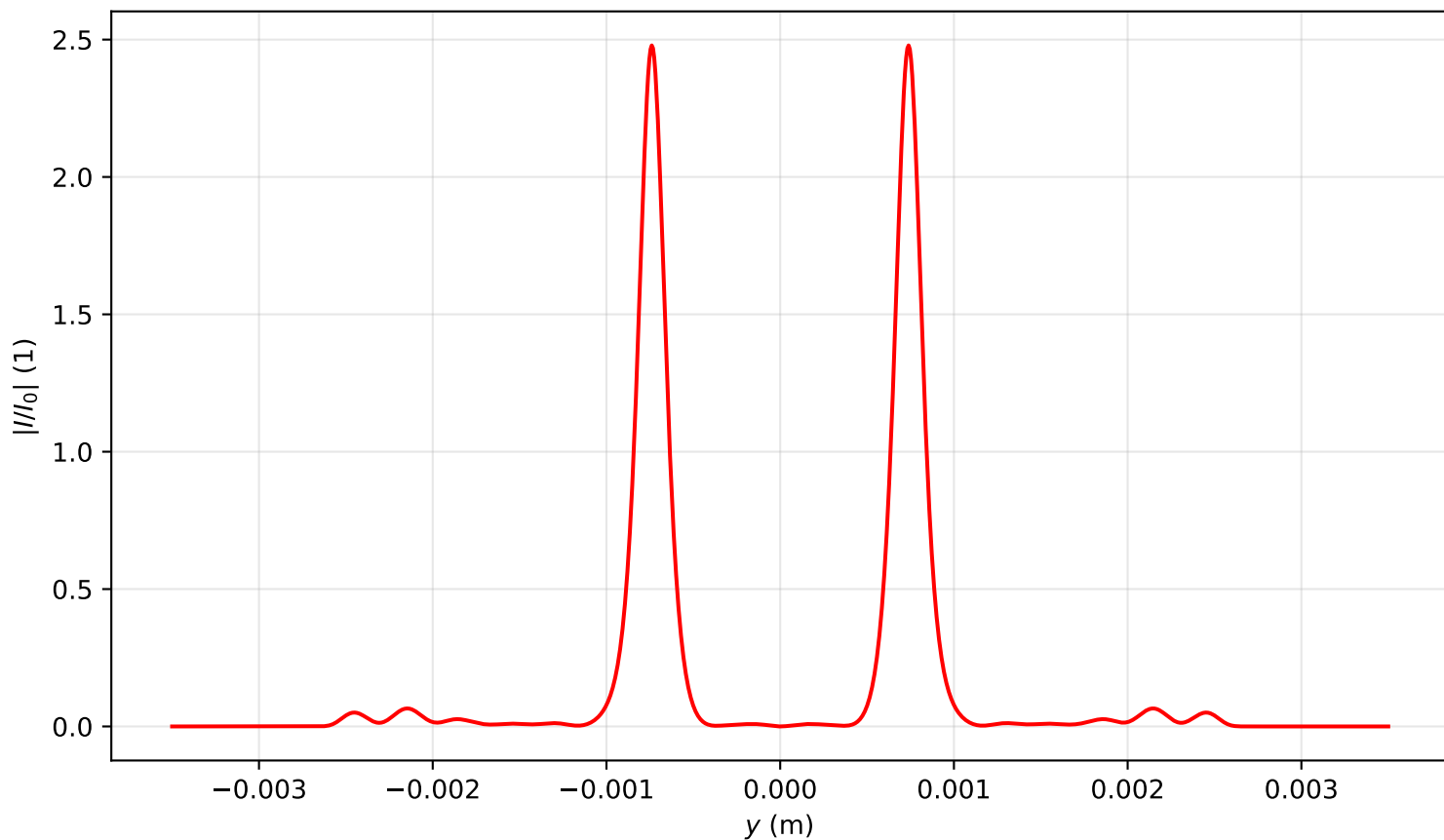
Intensity profile I(x=0, y, z=2.786)/I_0 , P_{in}=12.0P_{cr} , artificial time
