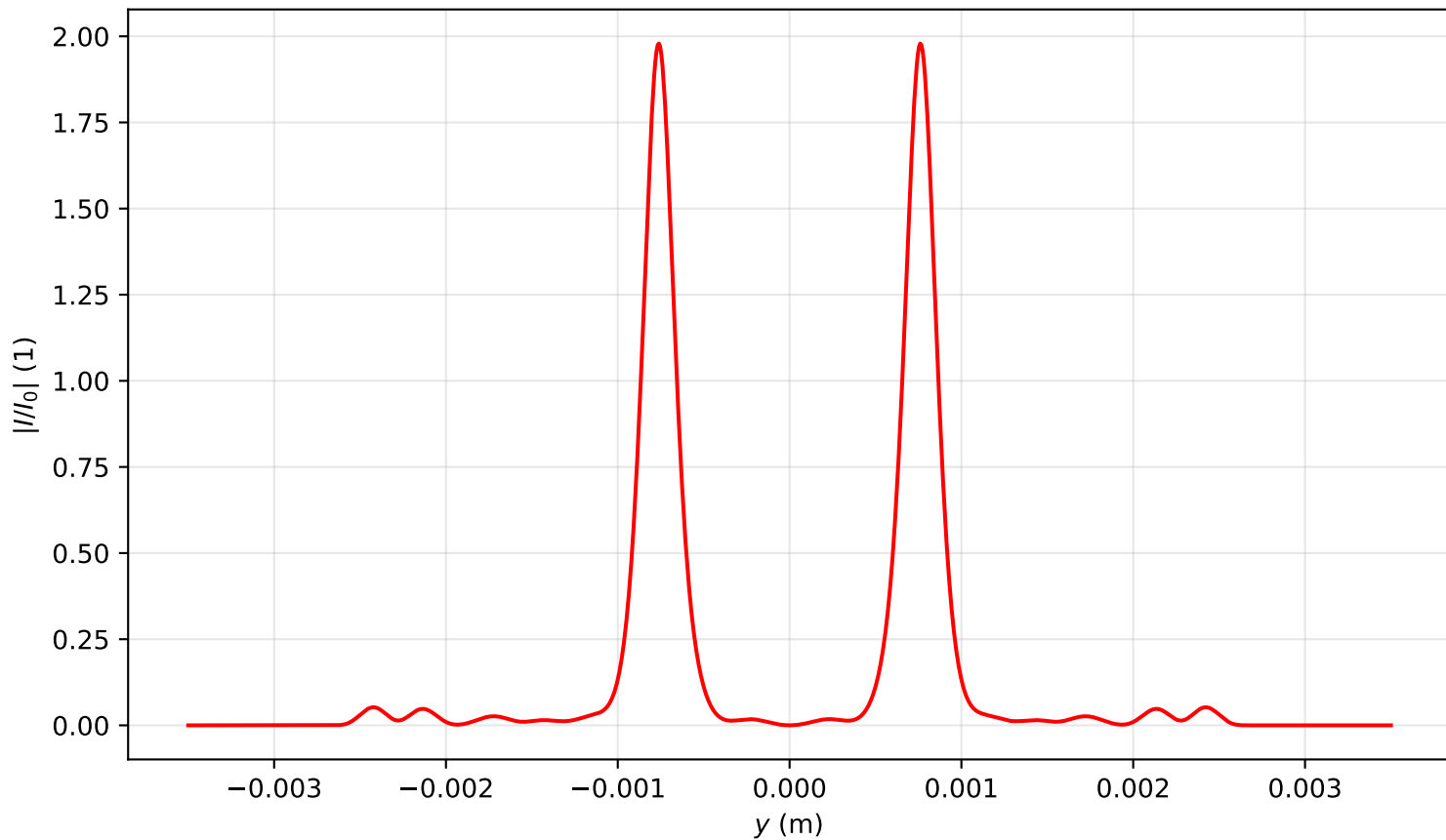
Intensity profile I(x=0, y, z=2.946)/I_0 , P_{in}=12.0P_{cr} , artificial time
