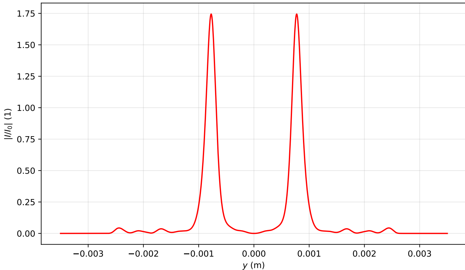
Intensity profile I(x=0, y, z=3.105)/I_0 , P_{in}=12.0P_{cr} , artificial time
