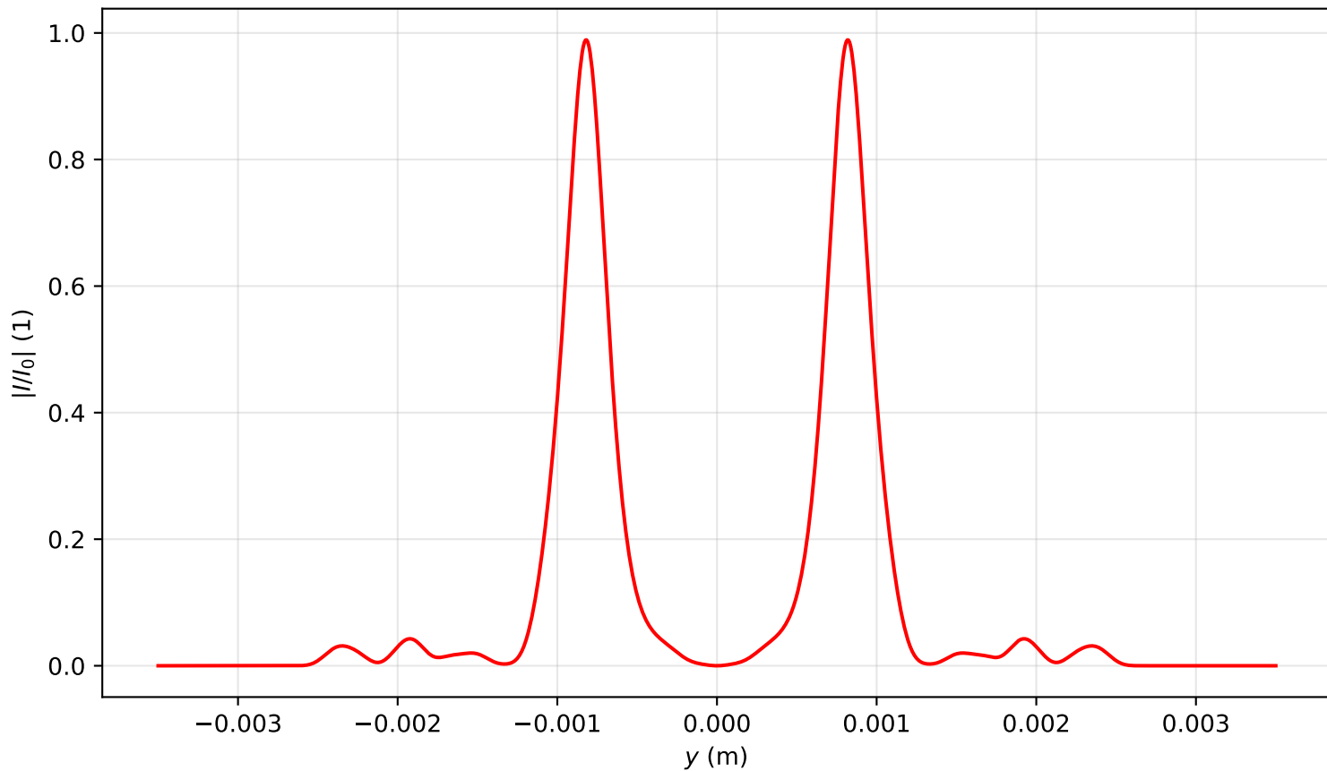
Intensity profile I(x=0, y, z=3.423)/I_0 , P_{in}=12.0P_{cr} , artificial time
