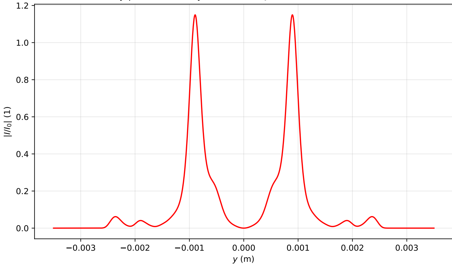
Intensity profile I(x=0, y, z=3.742)/I_0 , P_{in}=12.0P_{cr} , artificial time
