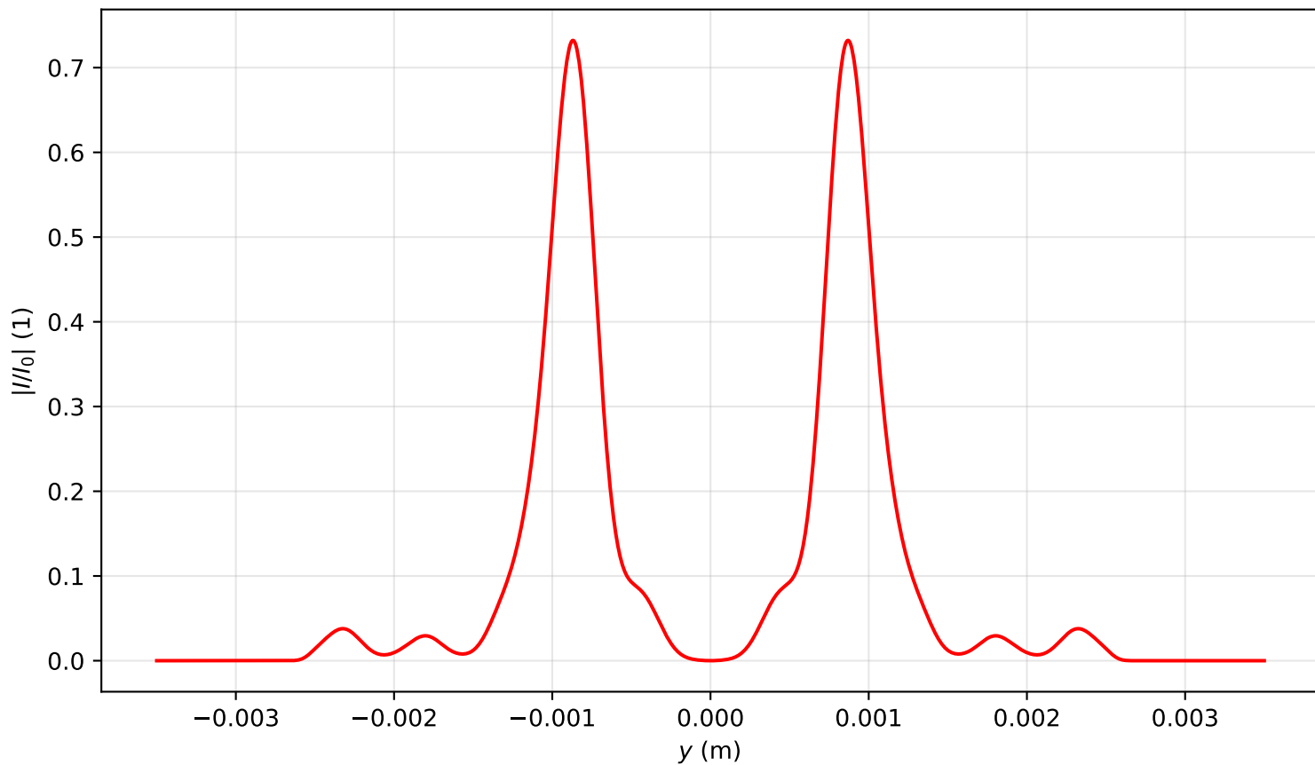
Intensity profile I(x=0, y, z=3.901)/I_0 , P_{in}=12.0P_{cr} , artificial time
