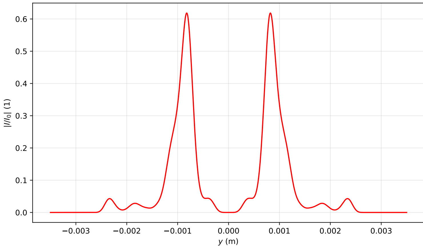
Intensity profile I(x=0, y, z=3.981)/I_0 , P_{in}=12.0P_{cr} , artificial time
