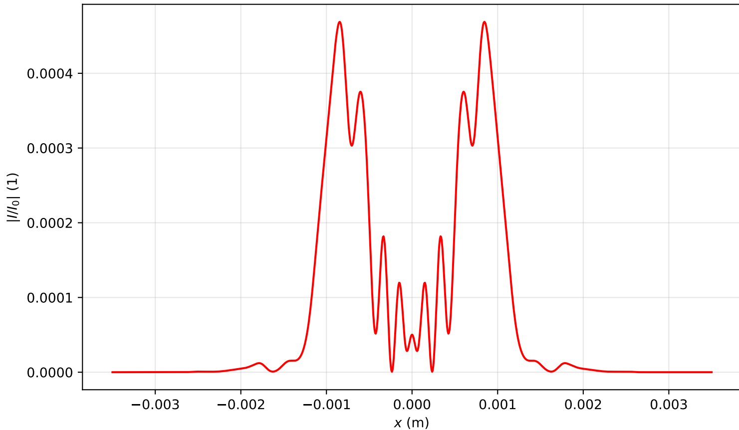
Intensity profile I(x, y = 0, z = 0.796)/I_0 , P_{in}=13.0P_{cr} , artificial time
