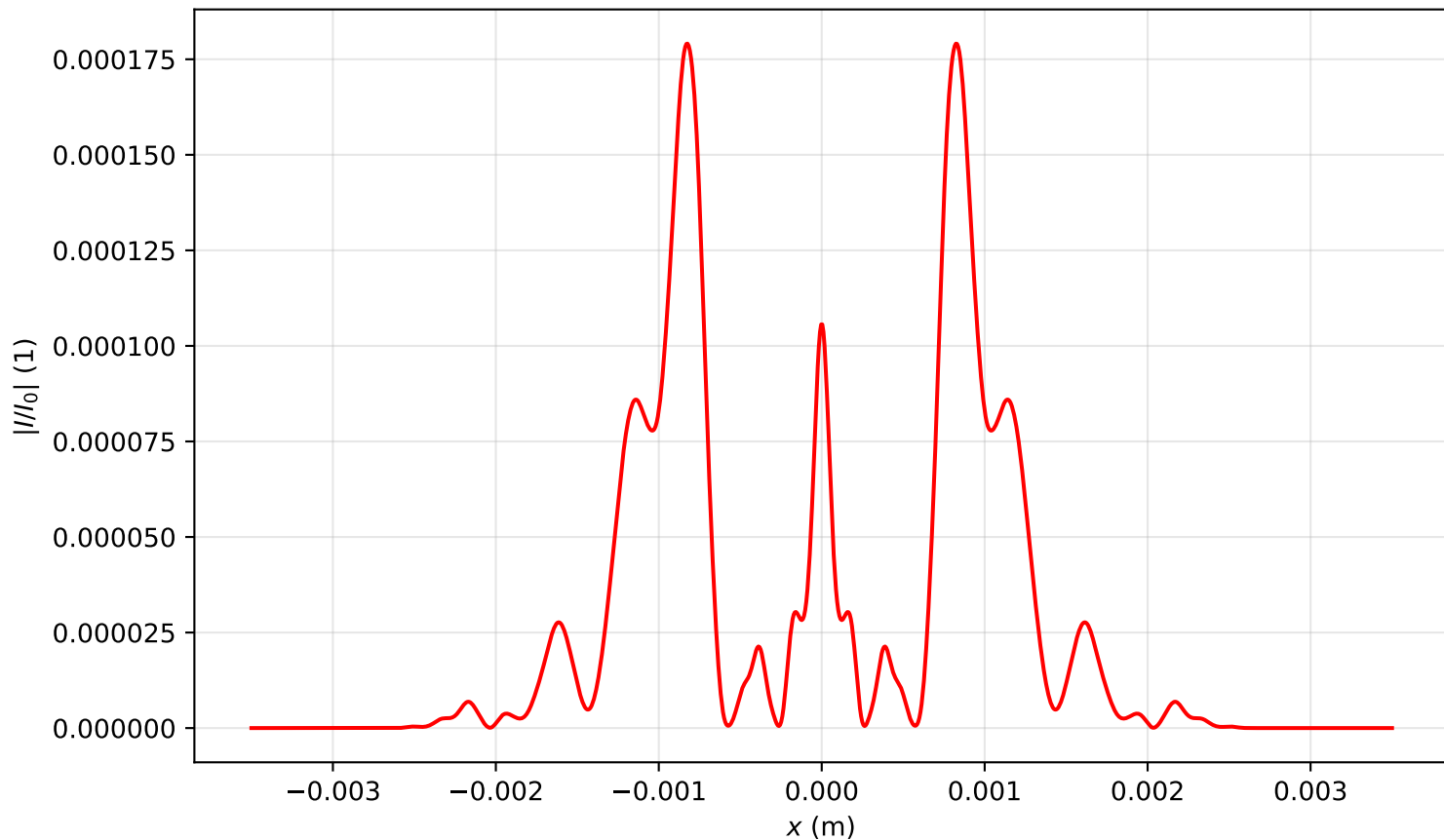
Intensity profile I(x, y = 0, z = 1.274)/I_0 , P_{in}=13.0\text{Pcr} , artificial time
