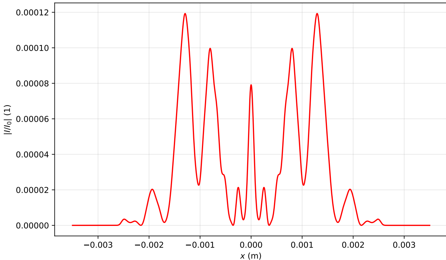
Intensity profile I(x, y = 0, z = 1.353)/I_0 , P_{in}=13.0P_{cr} , artificial time
