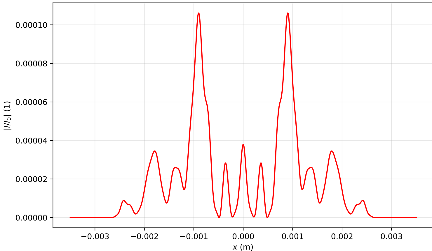
Intensity profile I(x, y = 0, z = 1.513)/I_0 , P_{in}=13.0P_{cr} , artificial time
